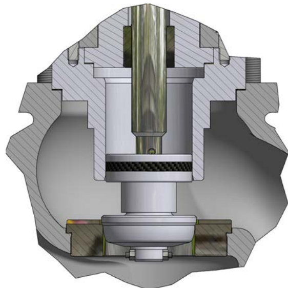
BALANCED TRIM
