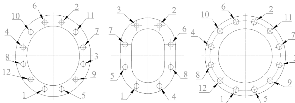
Fig. 5 Recommended re-tighten order
